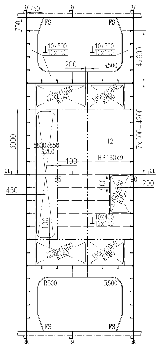
4970 PLATFORM 1:100
